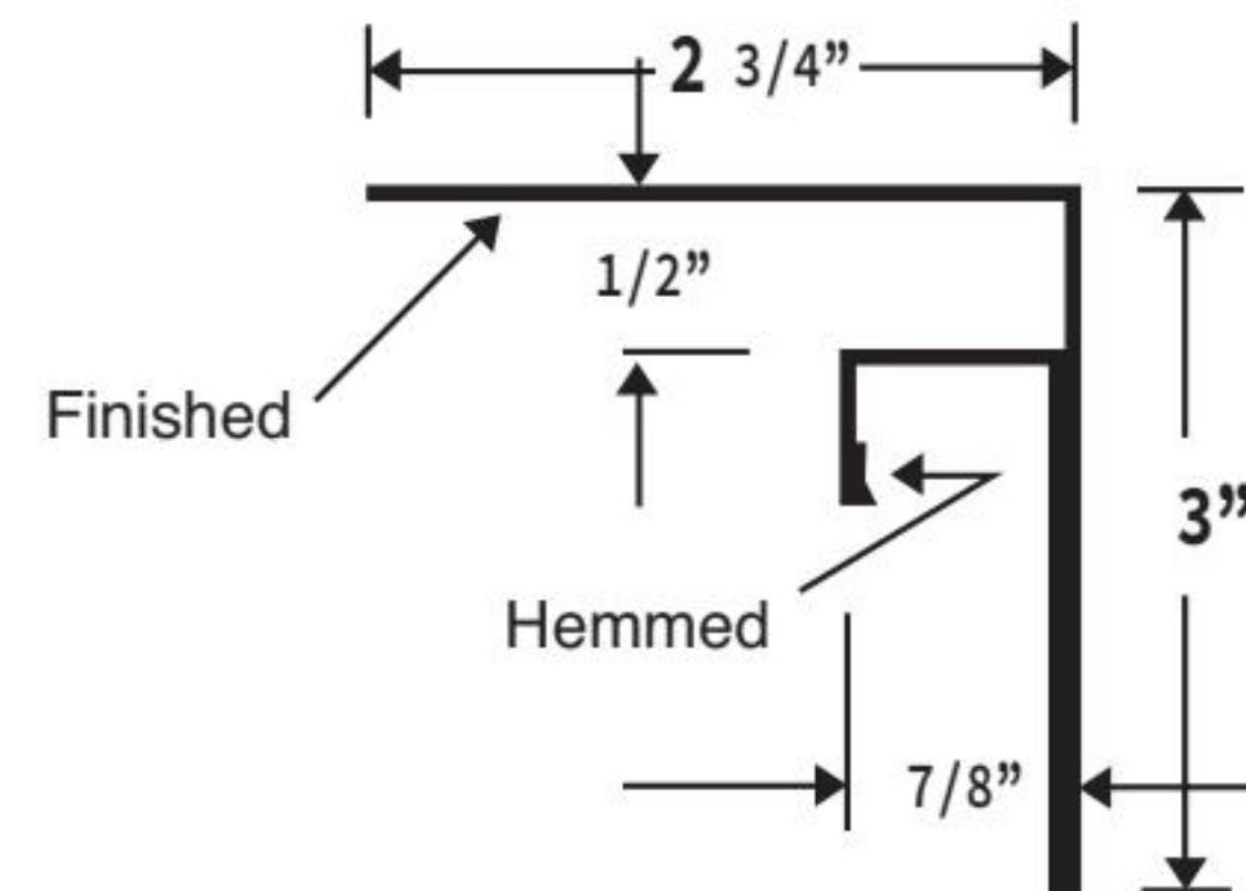
1/2" DOUBLE J TRIM
