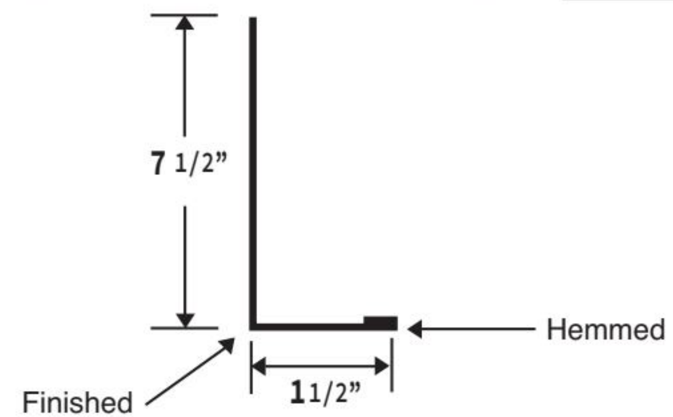
7 1/2" FASCIA / POST TRIM
