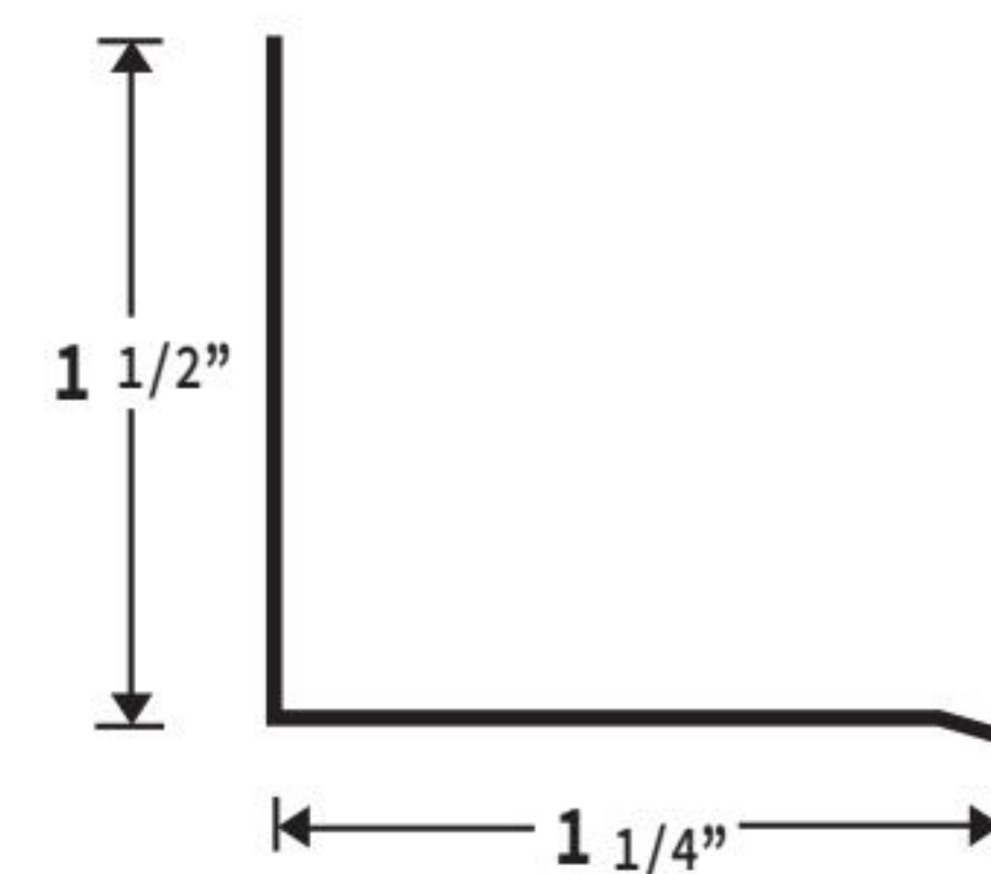
DRIP CAP TRIM
