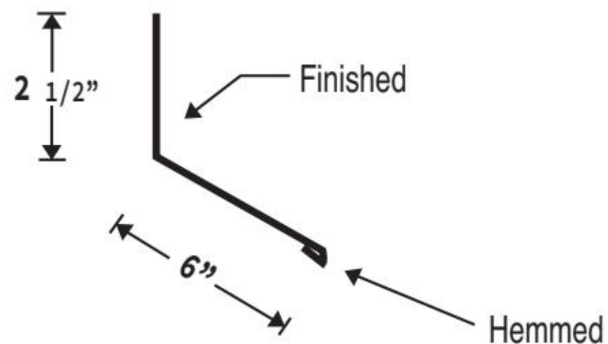
6" ENDWALL SIDEWALL
