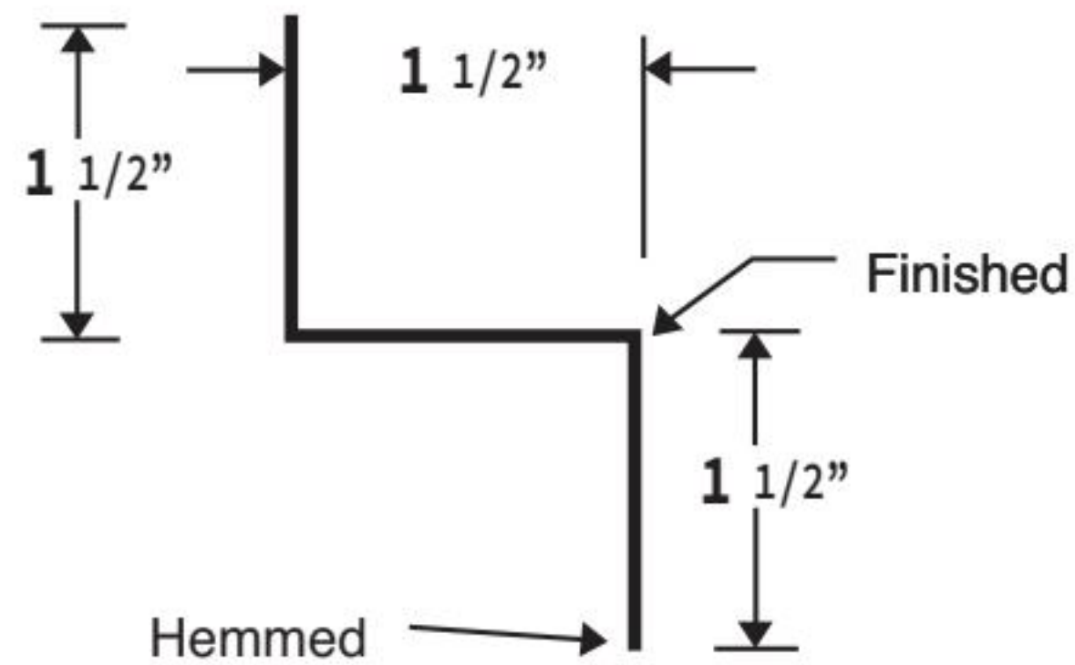
1 1/2" DOUBLE ANGLE
