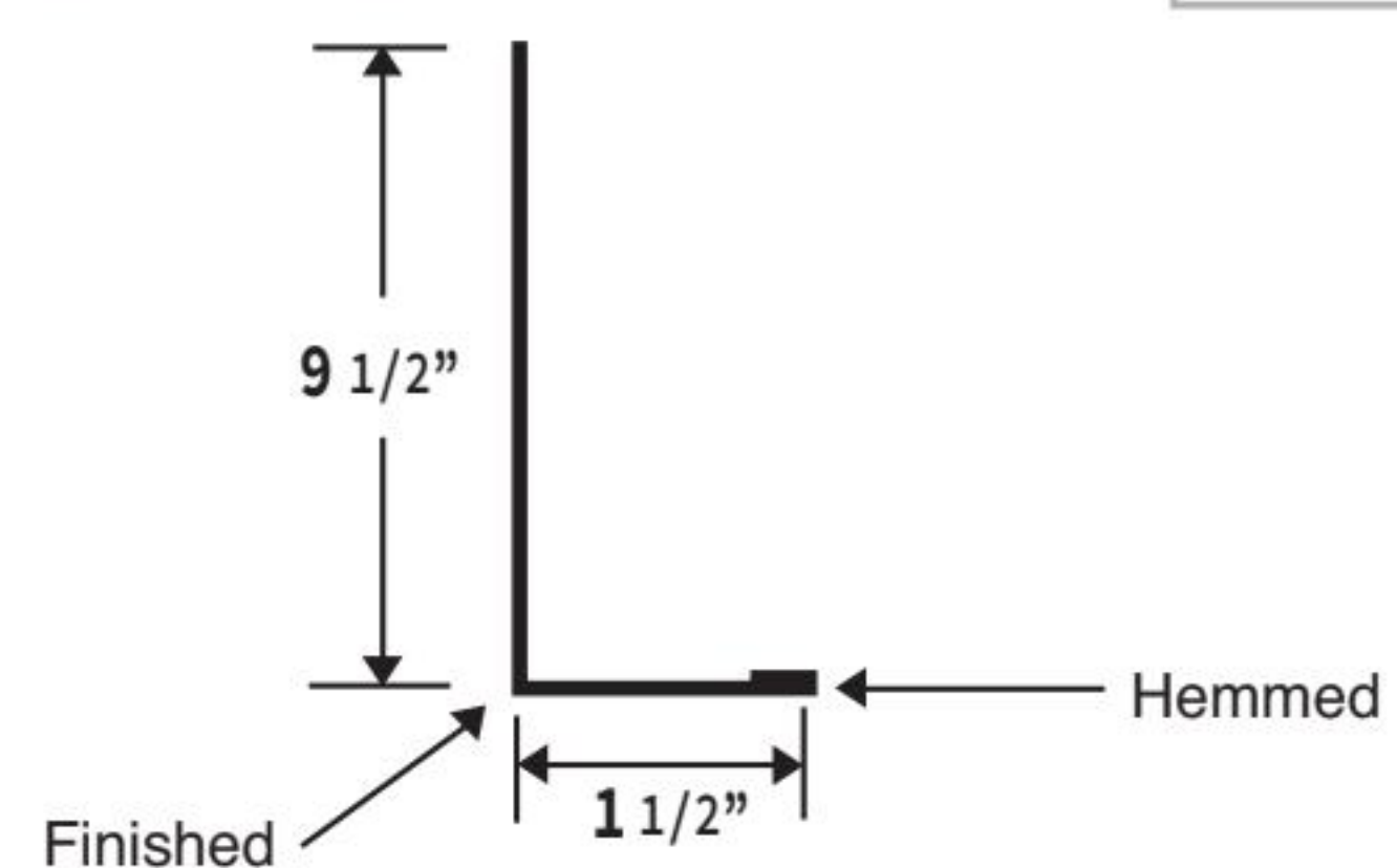
9 1/2" FASCIA / POST TRIM
