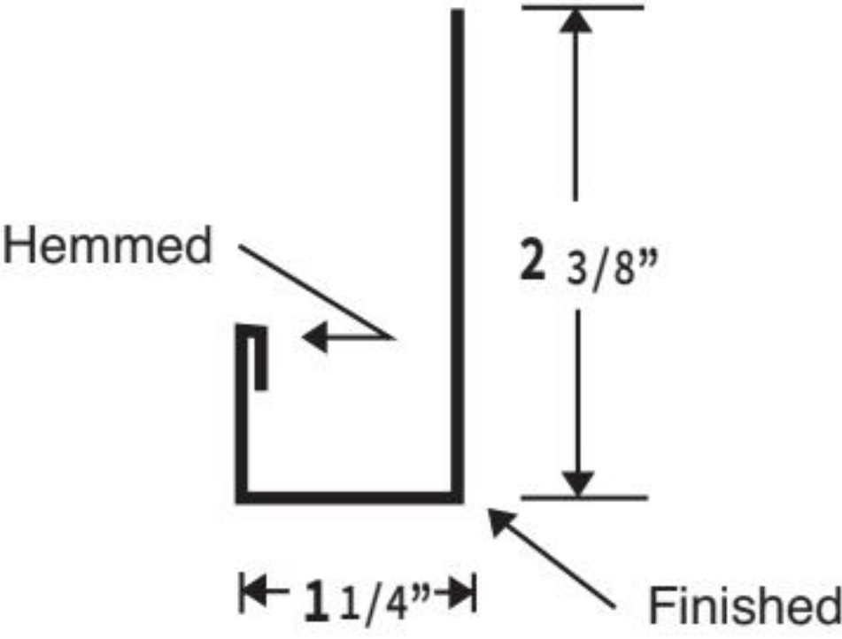
1 1/4" J TRIM
