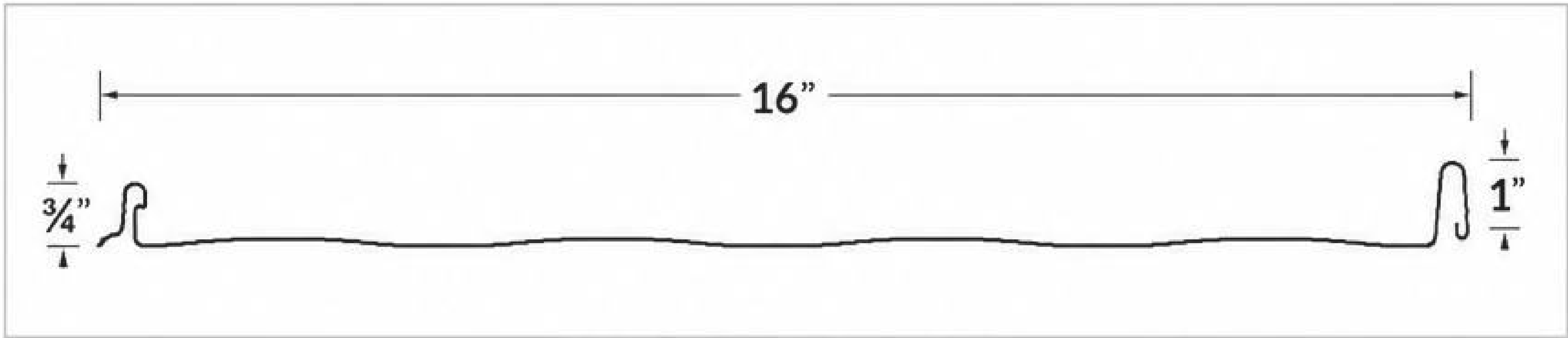
SnapLok 100 - profile cross-section
