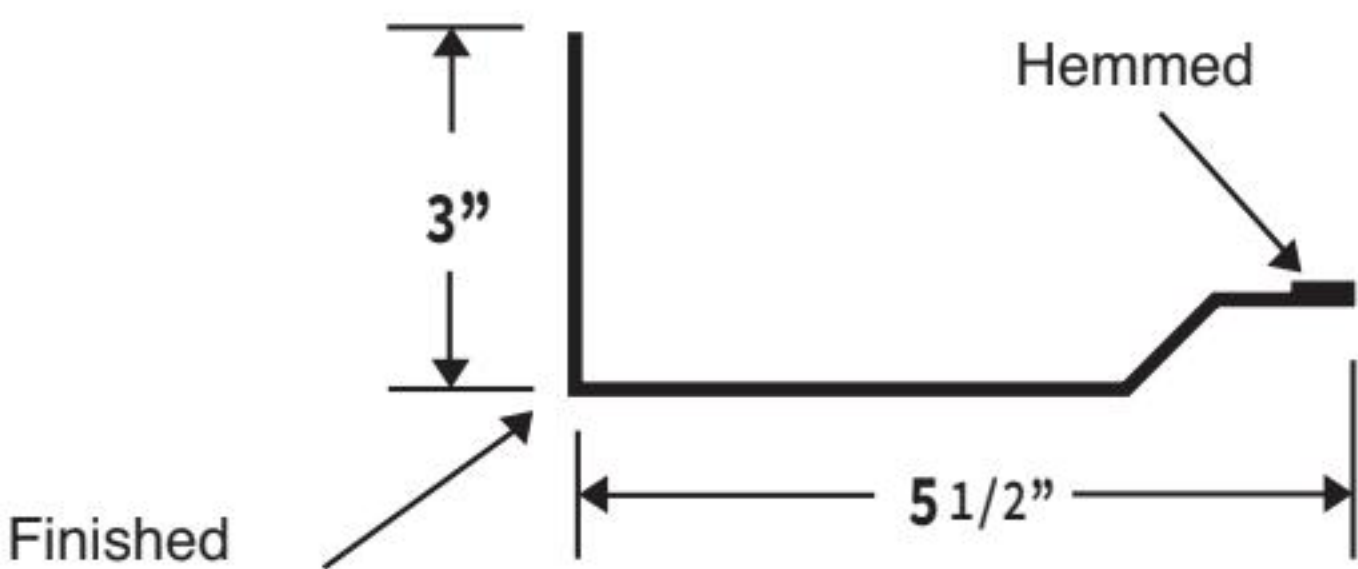
UNIVERSAL RAKE
