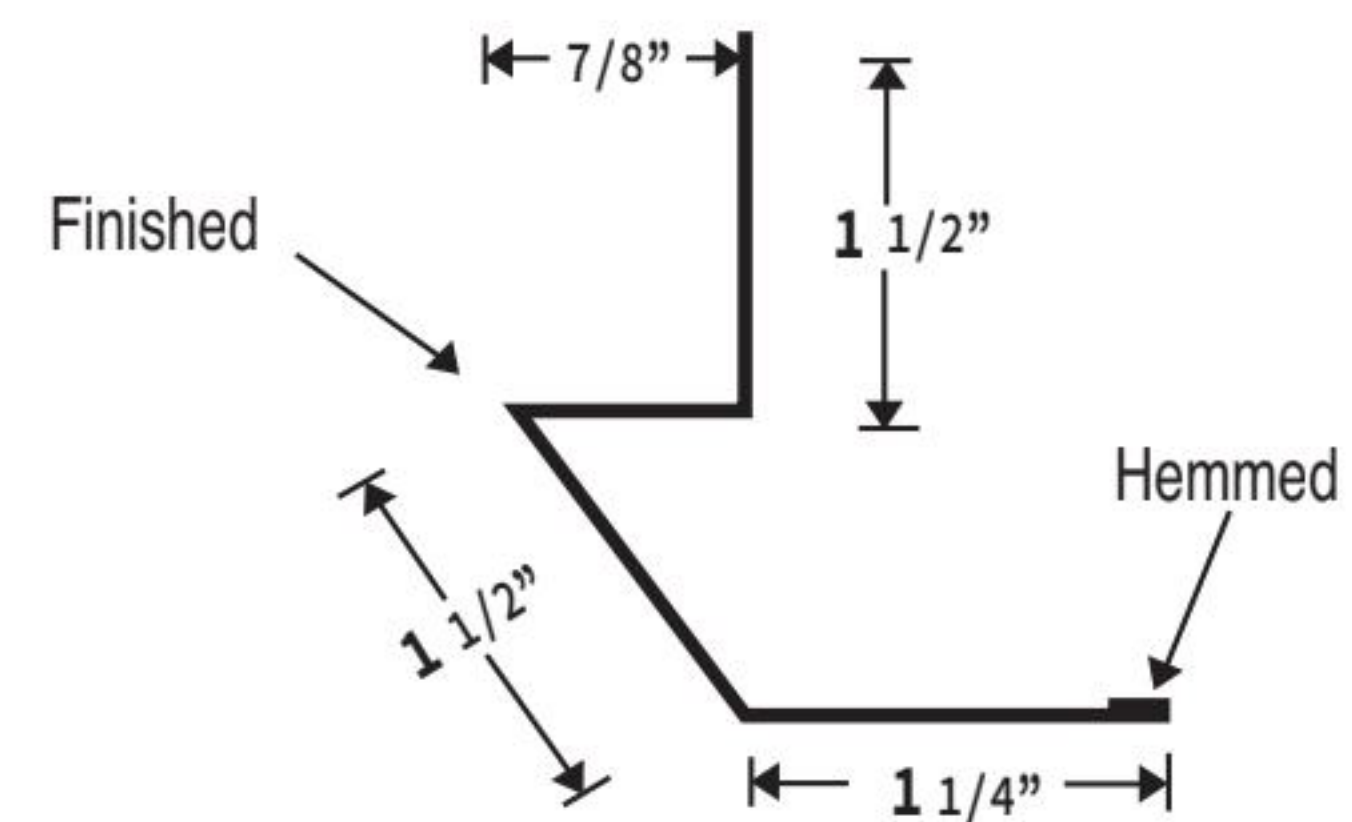
FLOATING BASE TRIM
