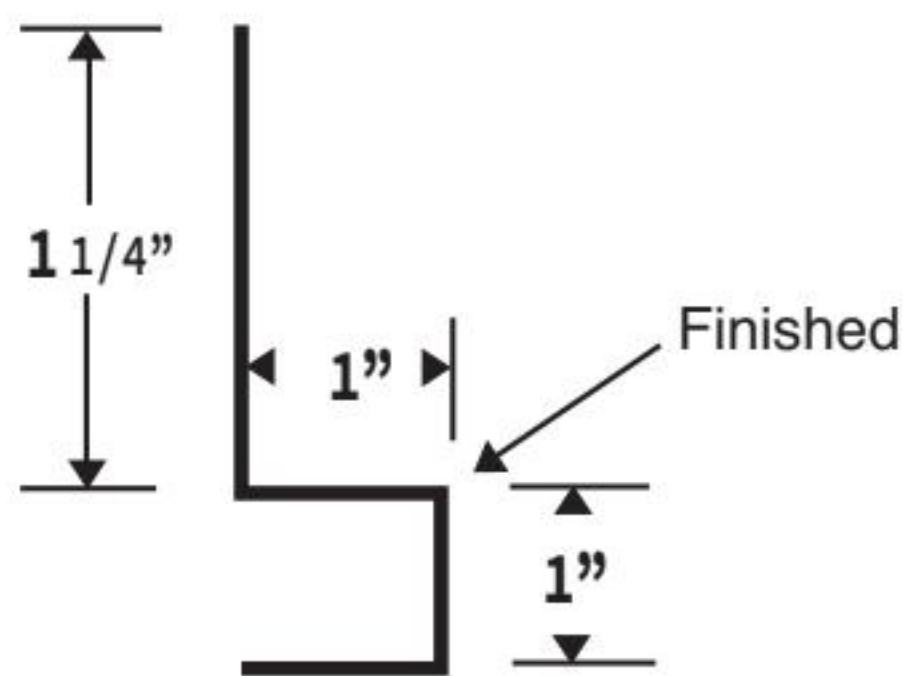
STARTER STRIP
