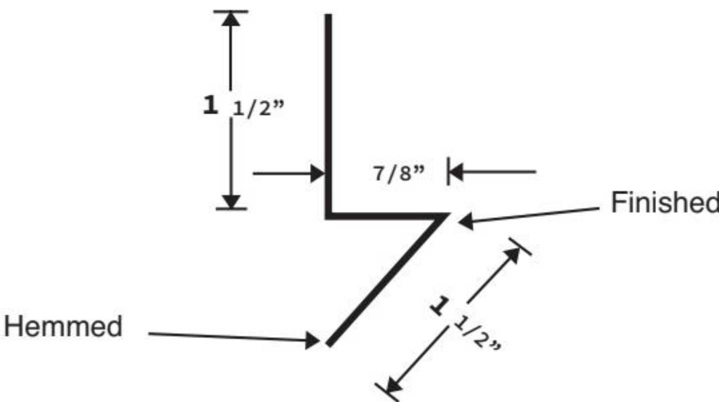
RAT GUARD
