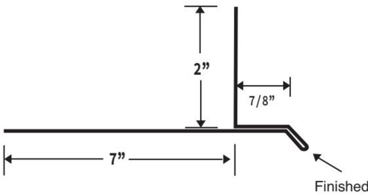
7" OVERHEAD DOOR WITH DRIP
