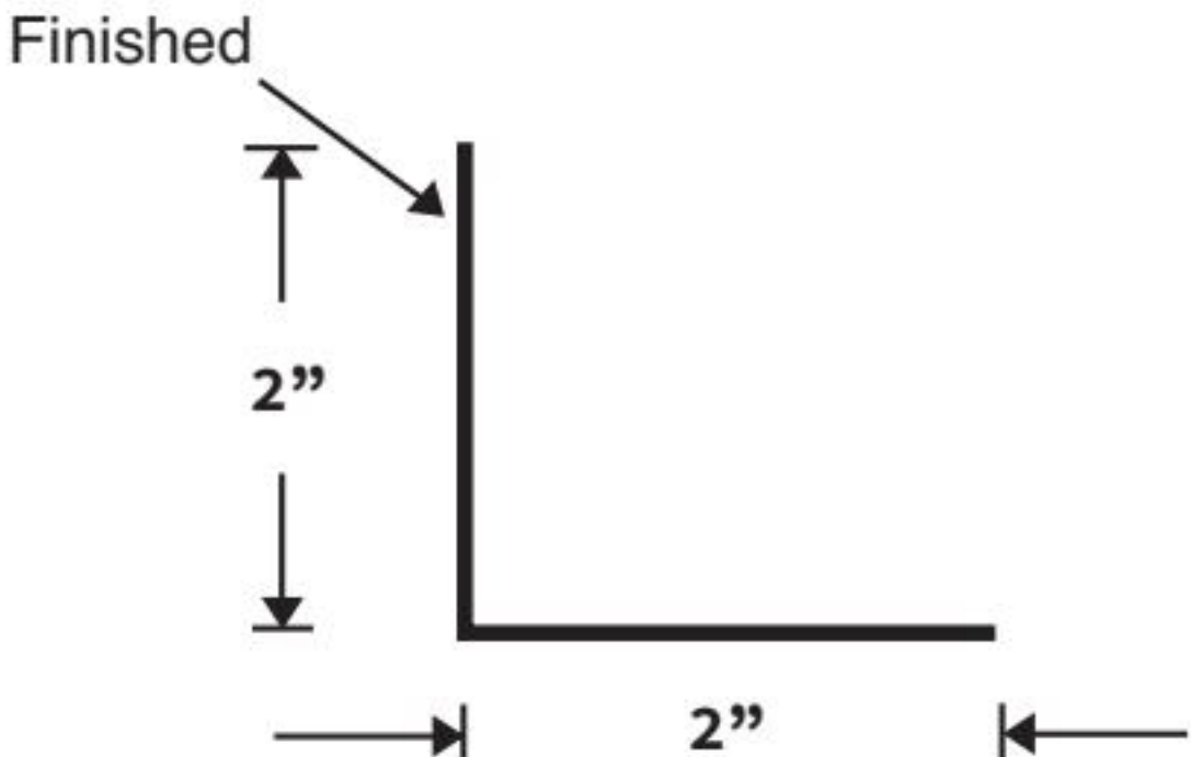
2" ANGLE FLASHING
