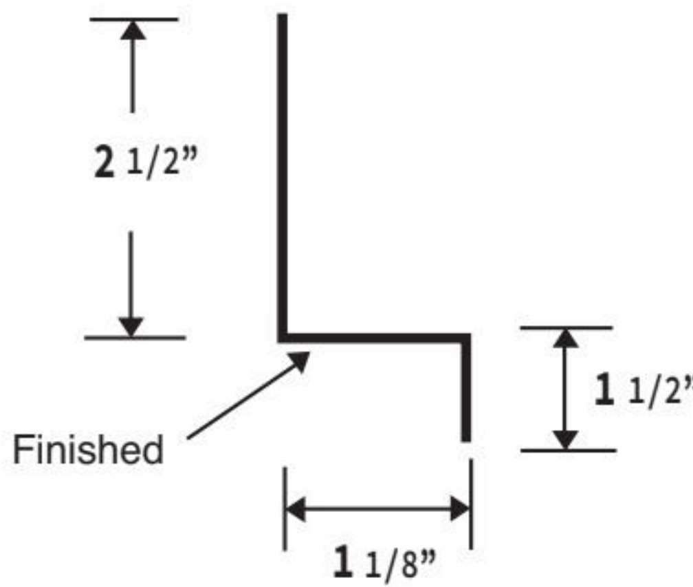
TRACK BOARD COVER
