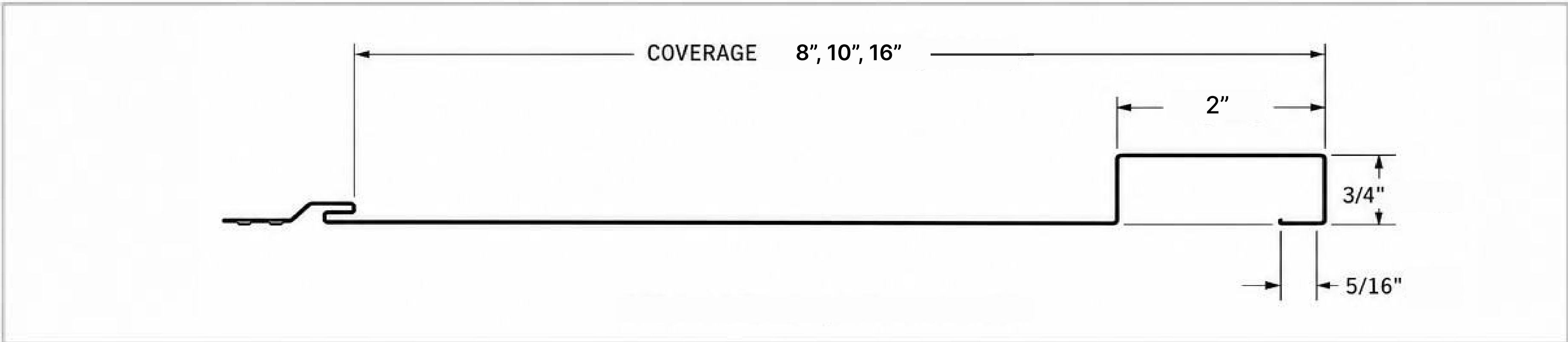
8" Board & Batten - profile cross-section
