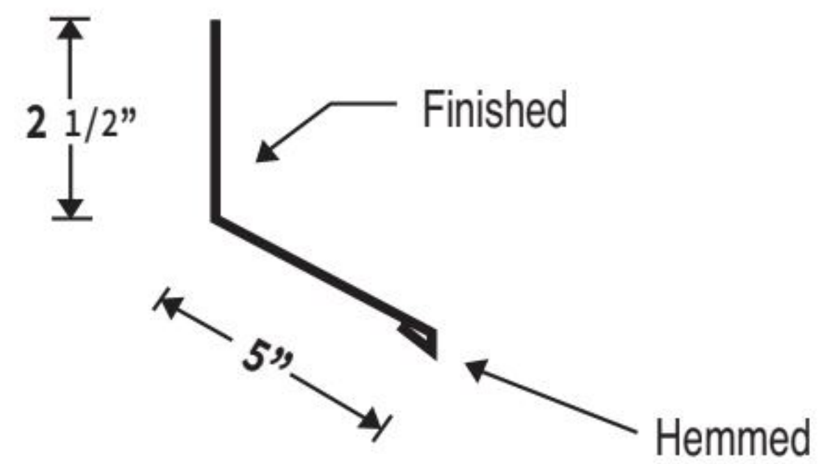
5" ENDWALL SIDEWALL
