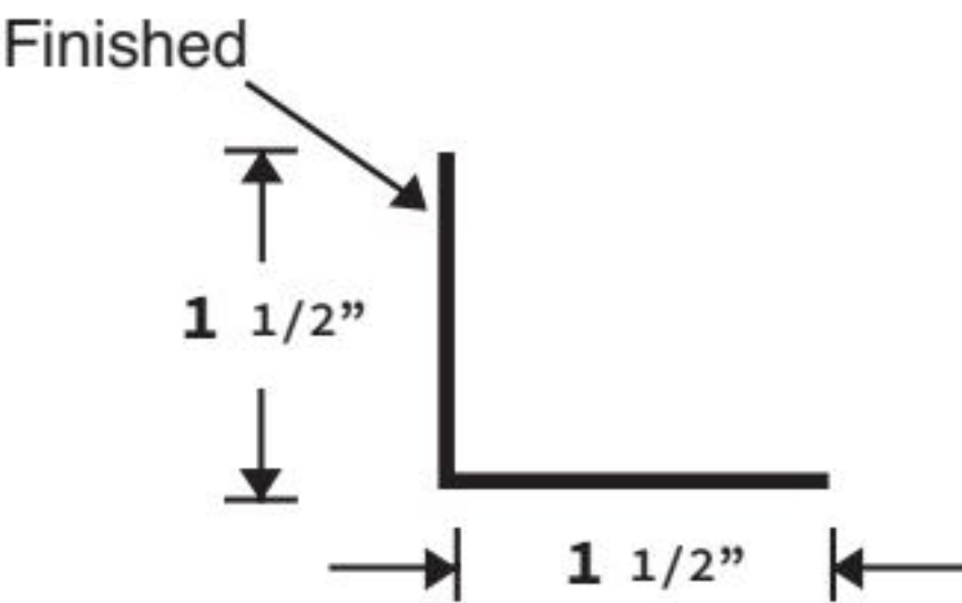
1 1/2" ANGLE FLASHING
