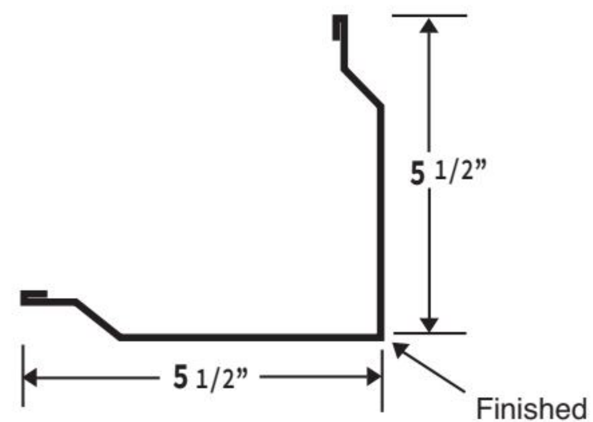
5" X 5" RAKE & CORNER
