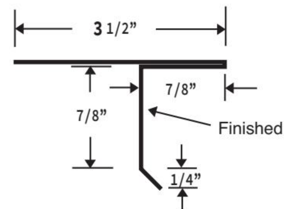
ROOF EDGE W/ DRIP
