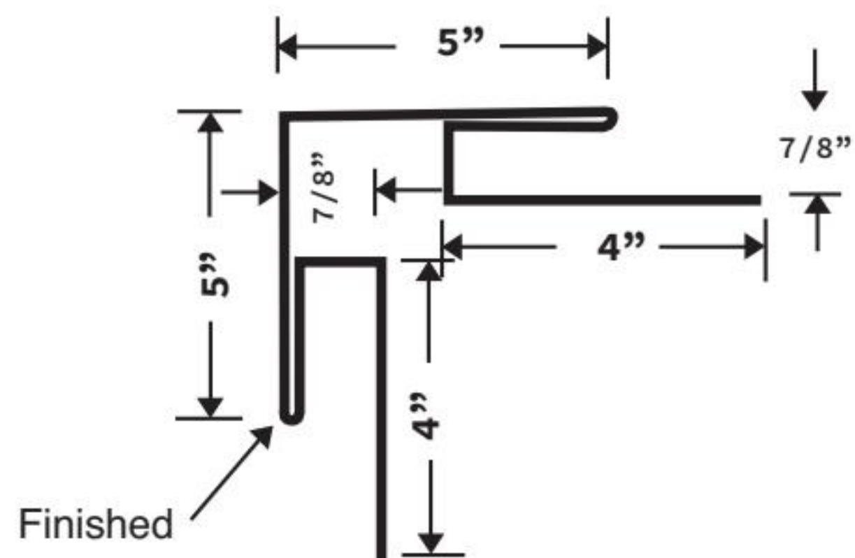
CLASSIC CORNER TRIM
