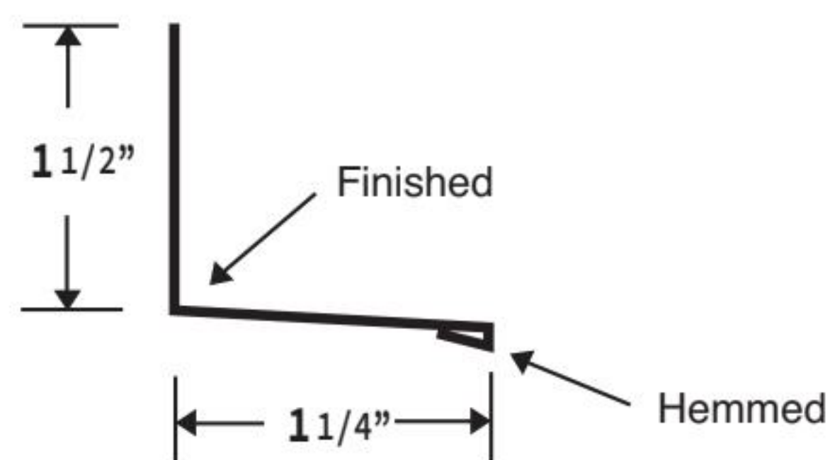
SIDEWALL FLASHING
