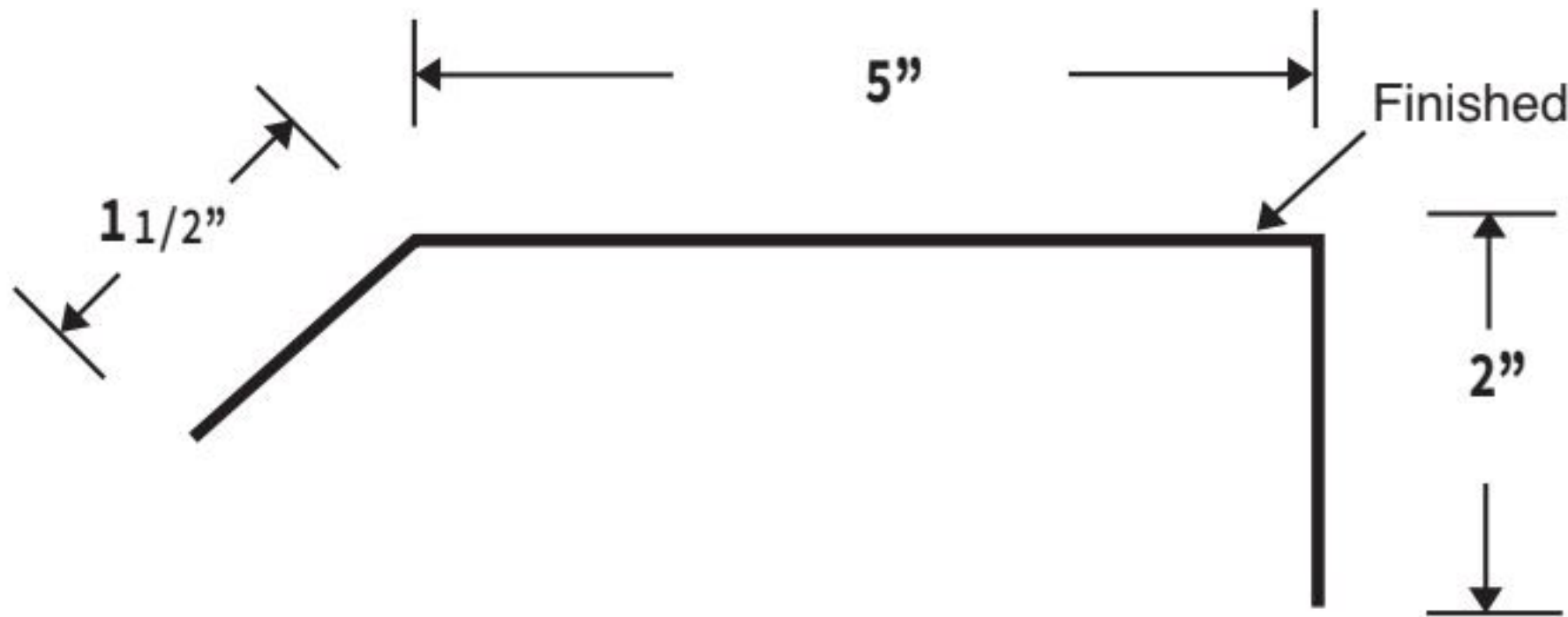
6" HOG BARN SNOW GUARD
