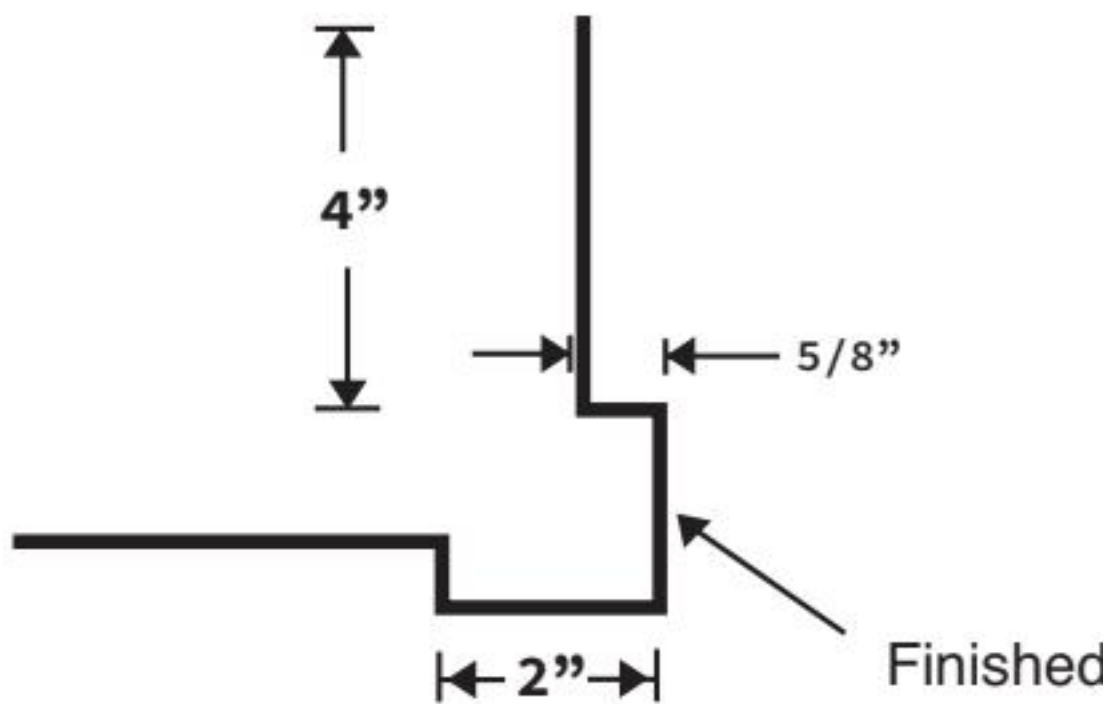
BULL NOSE TRIM
