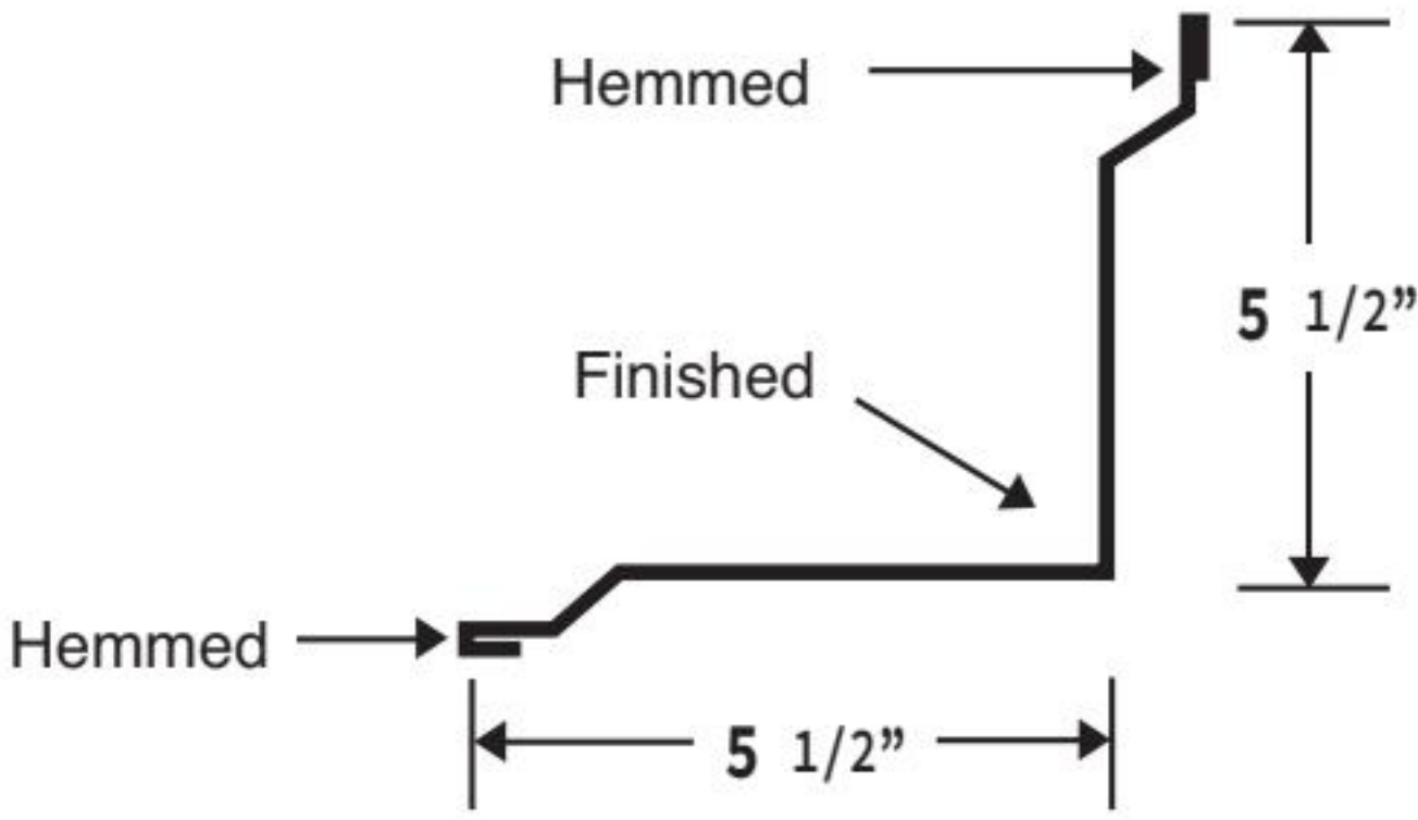
INSIDE CORNER
