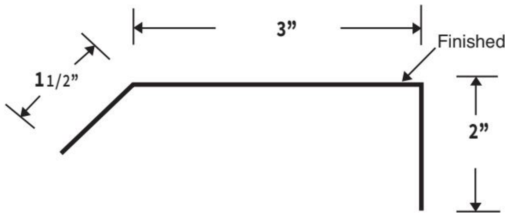
4" HOG BARN SNOW GUARD
