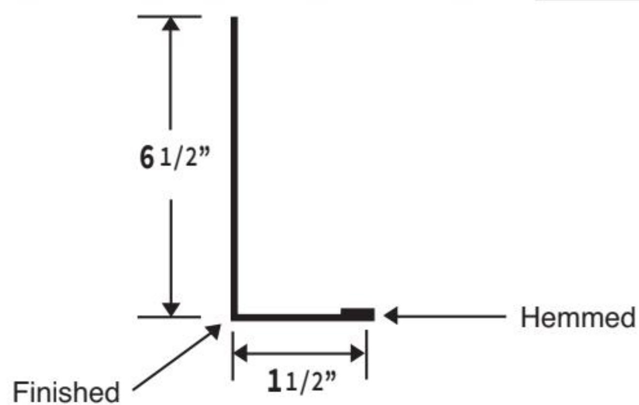
6 1/2" FASCIA / POST TRIM
