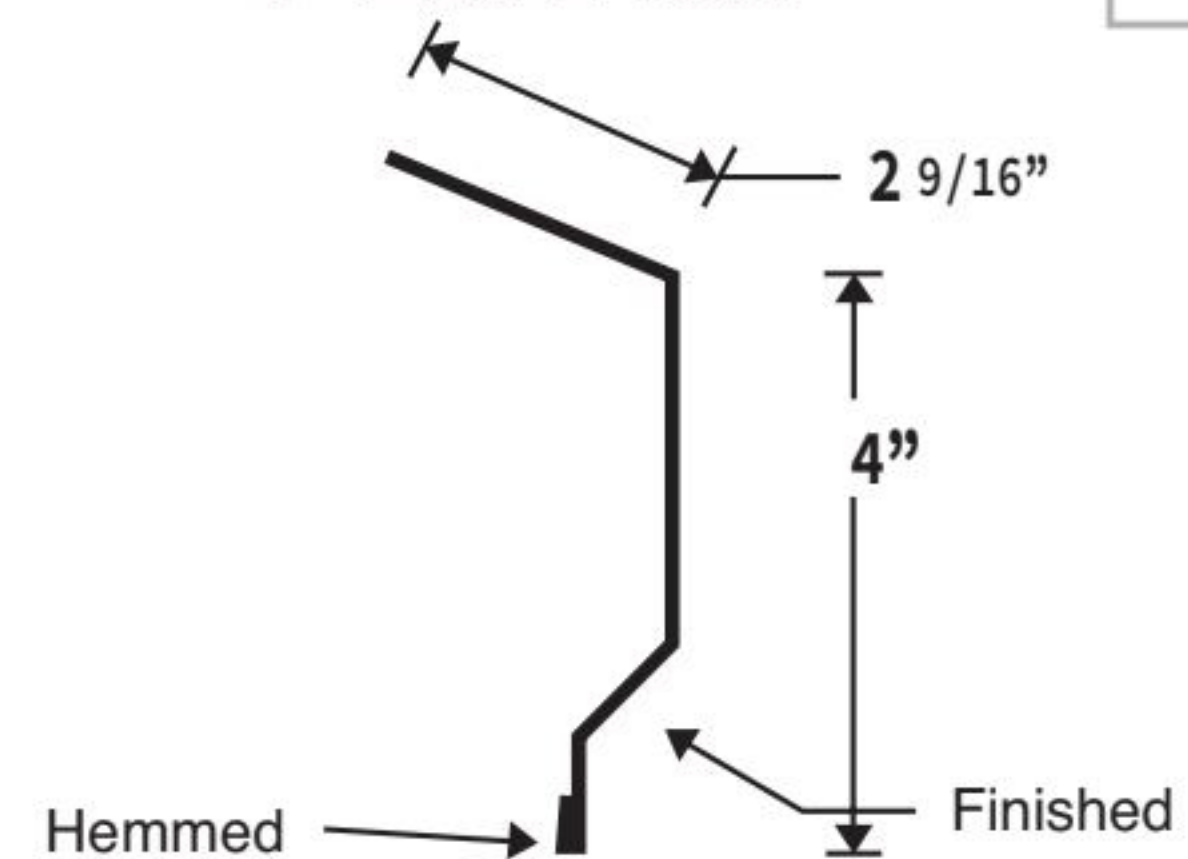
4" EAVE TRIP
