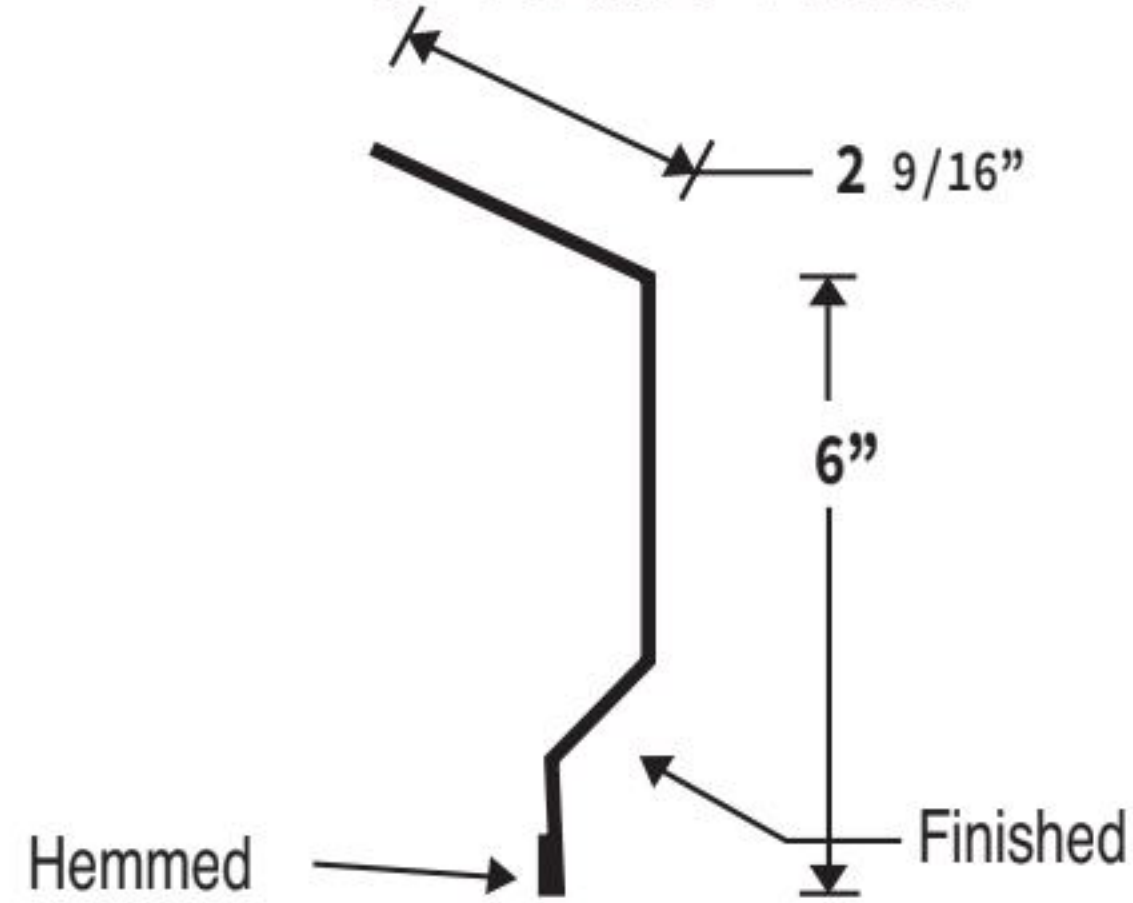
6" EAVE TRIM
