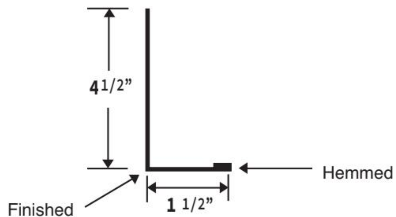
4 1/2" FASCIA / POST TRIM
