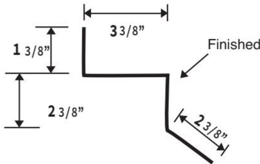
TRACK COVER
