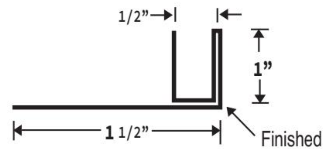
1/2" F TRIM
