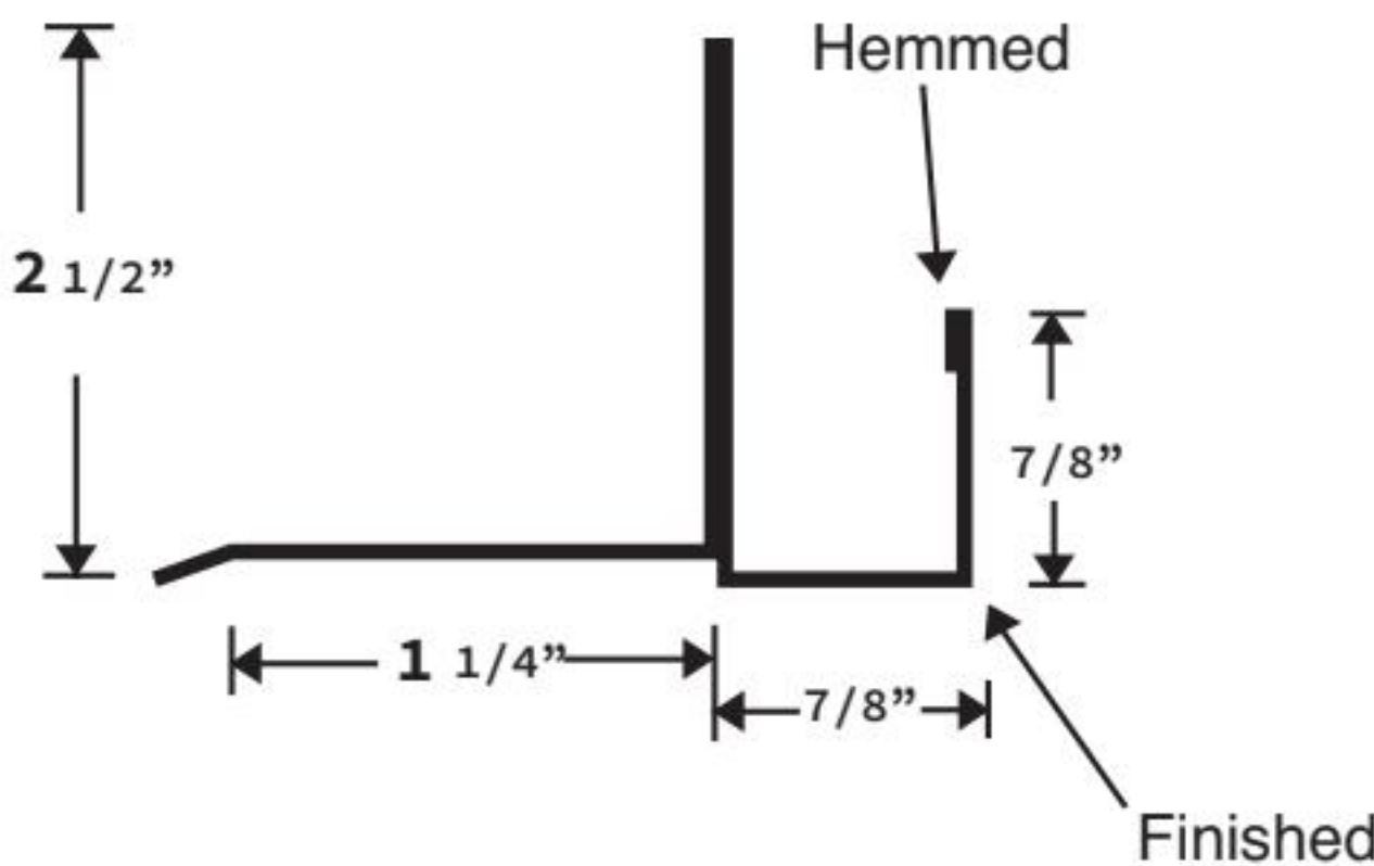
BOXED SOFFIT TRIM
