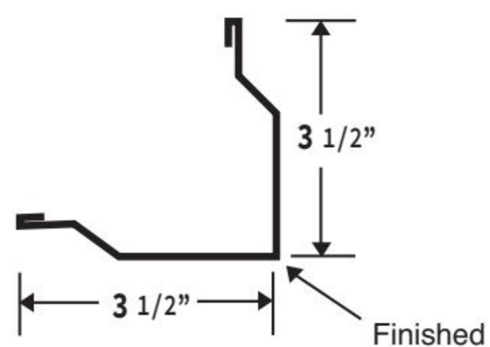
3" X 3" RAKE & CORNER
