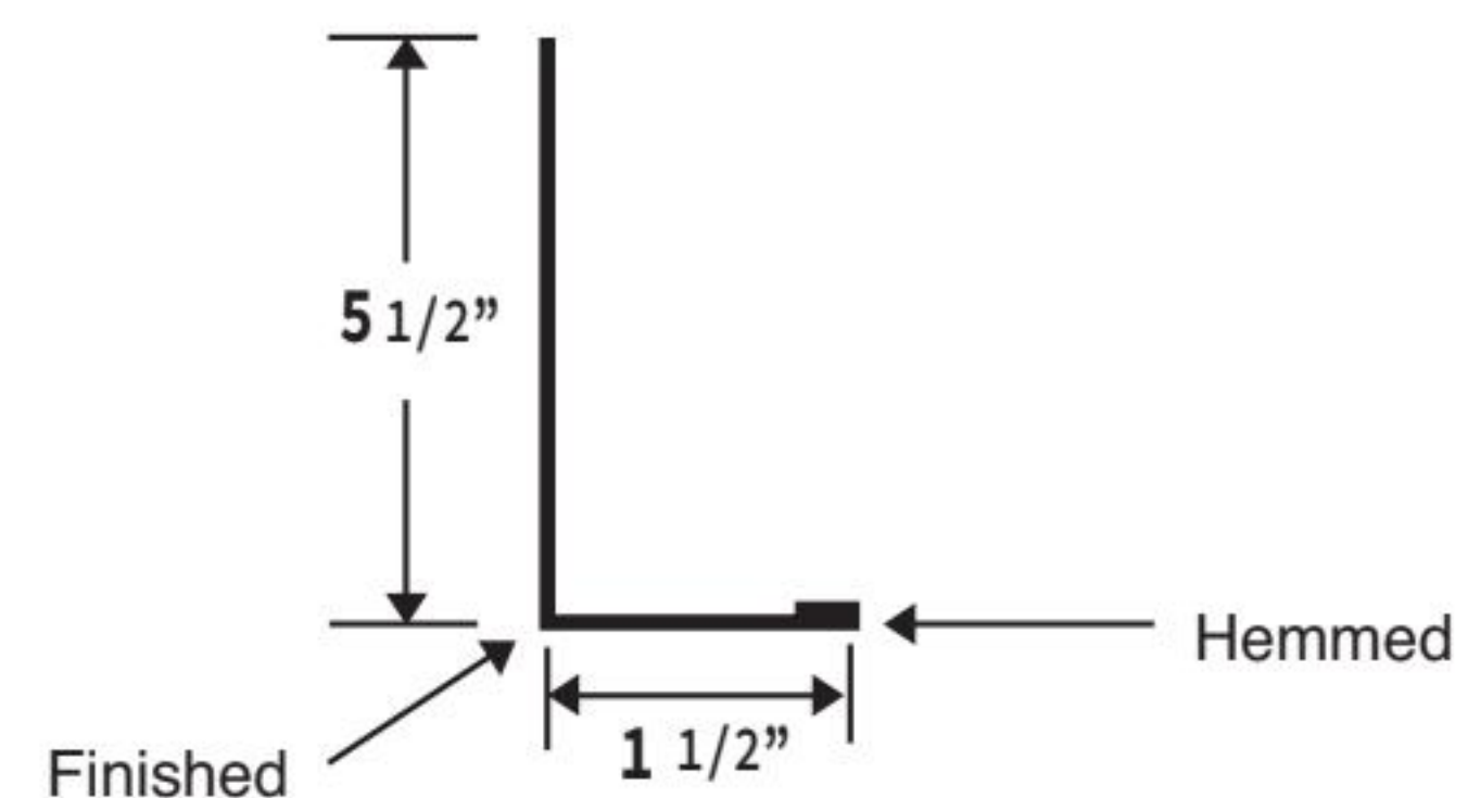
5 1/2" FASCIA / POST TRIM
