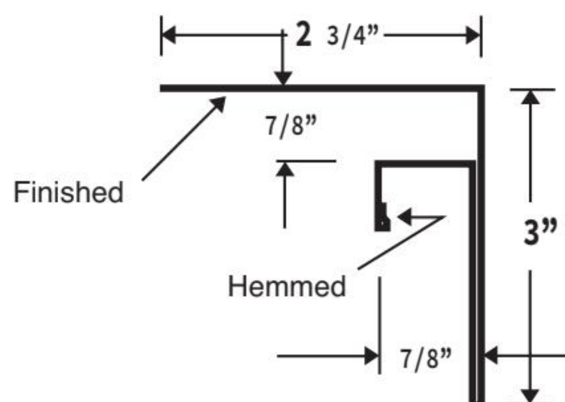
7/8" DOUBLE J TRIM
