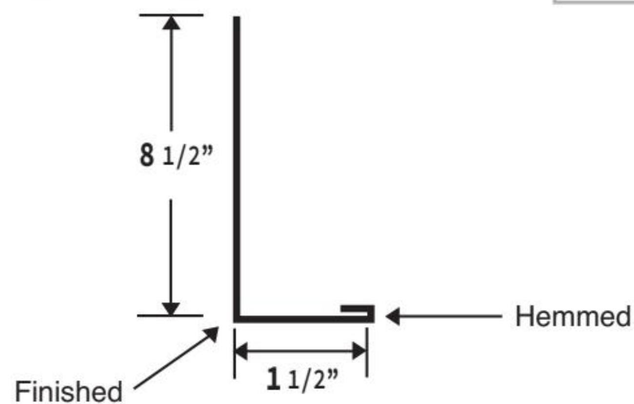
8 1/2" FASCIA / POST TRIM
