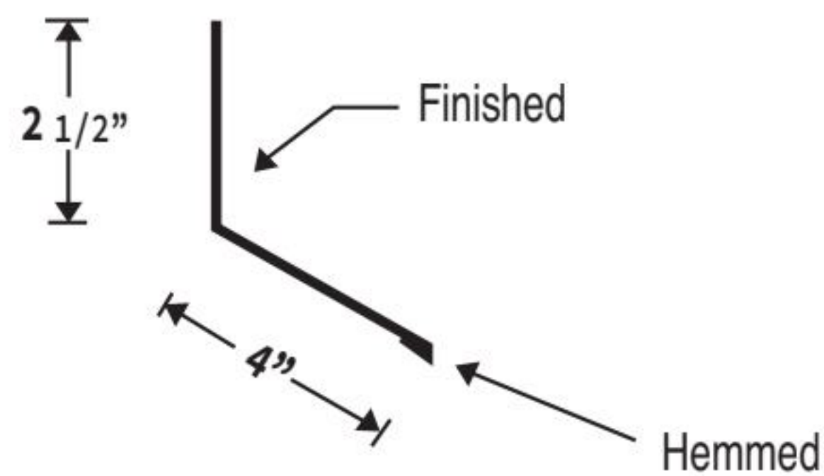
4" ENDWALL SIDEWALL
