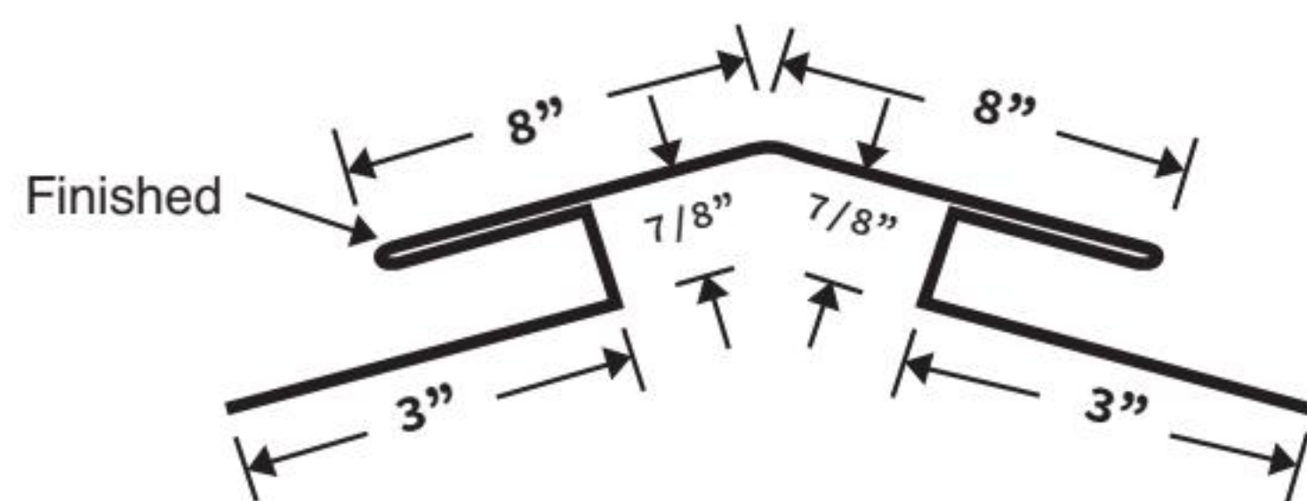
CLASSIC RIDGE CAP
