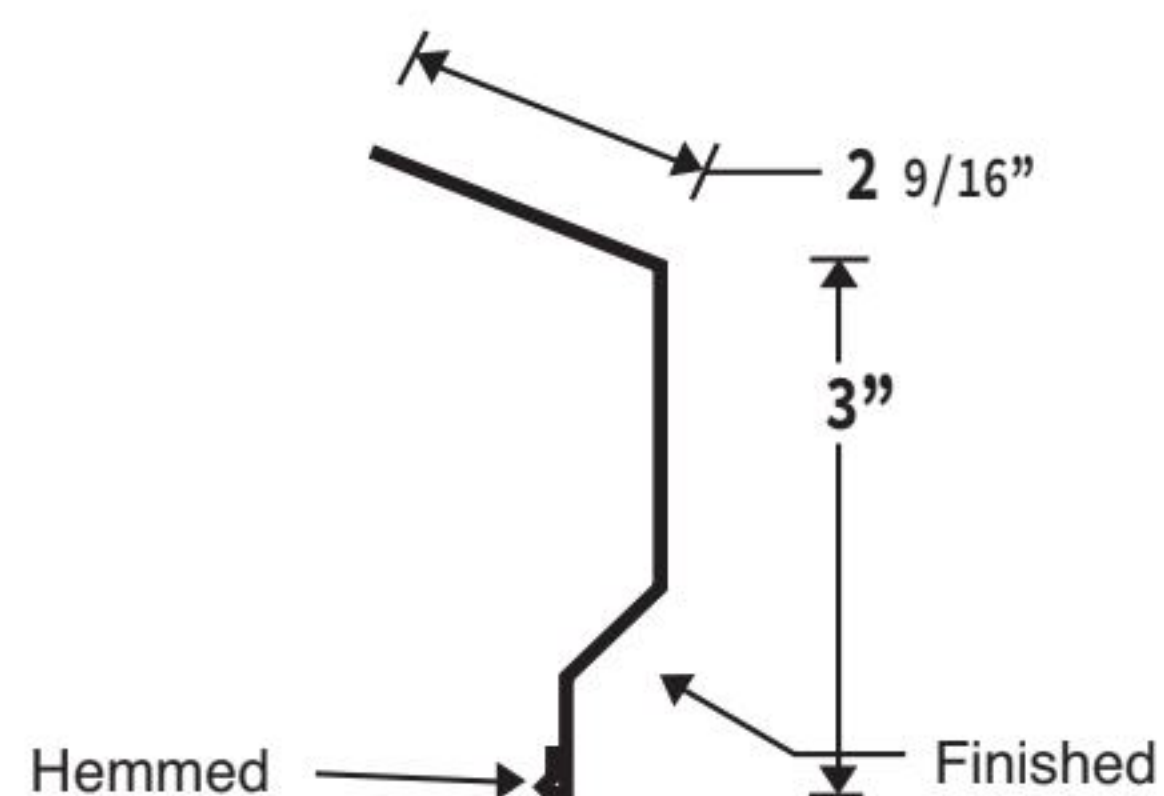
3" EAVE TRIP
