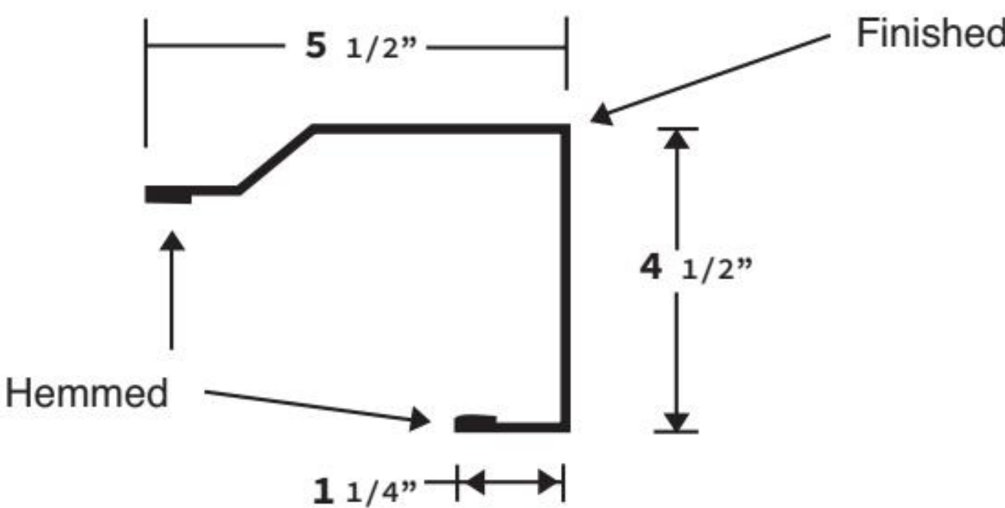
BULL NOSE TRIM
