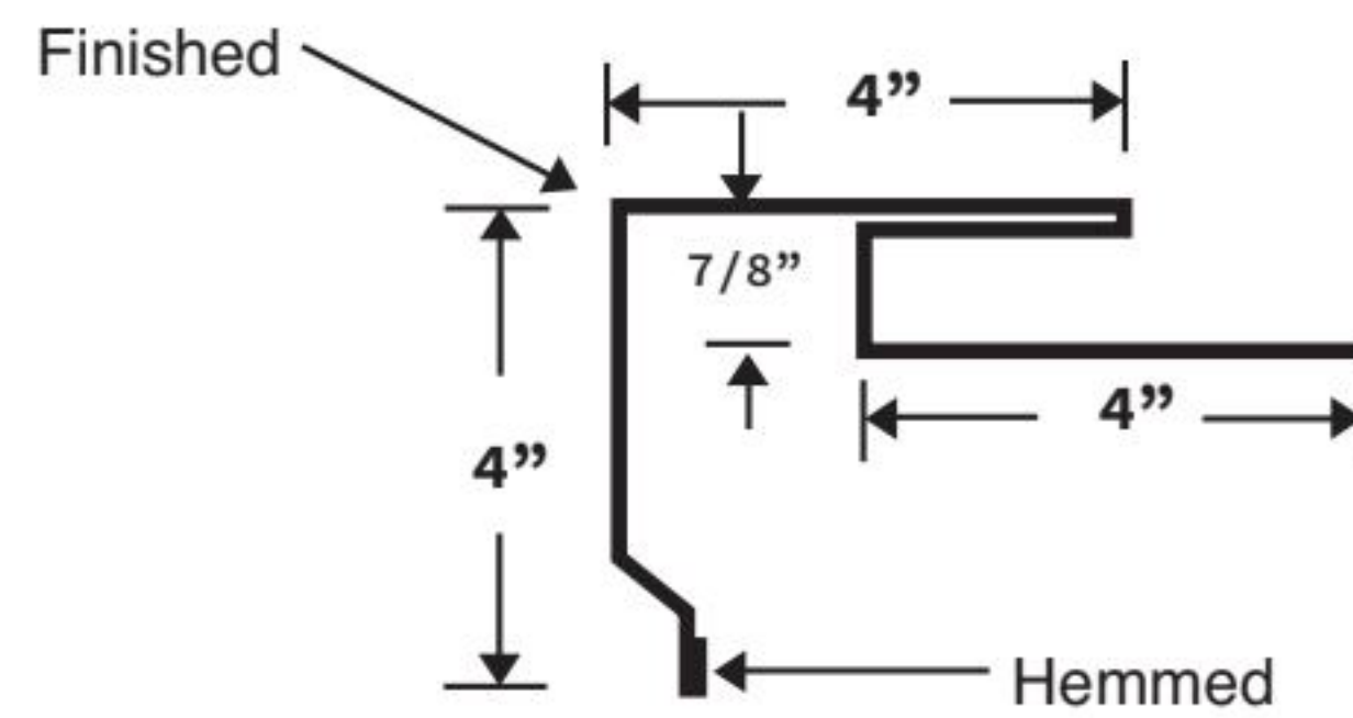
CLASSIC RAKE TRIM
