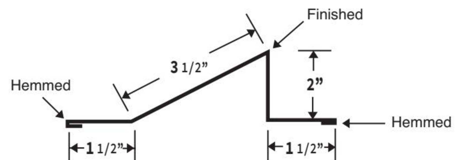
SNOW GUARD
