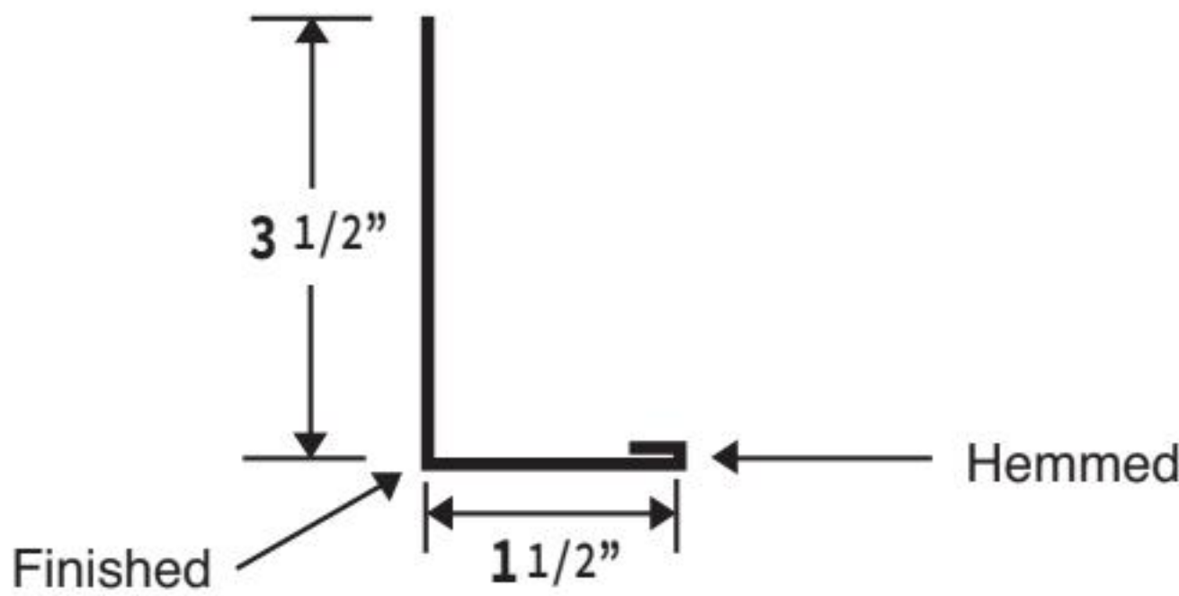
3 1/2" FASCIA / POST TRIM
