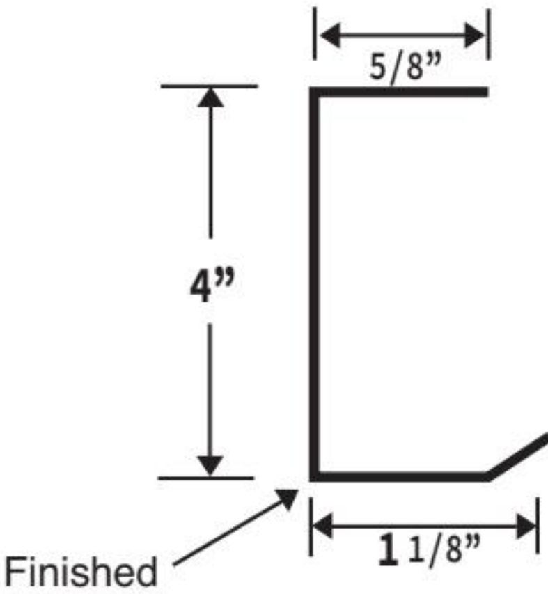
POST COVER
